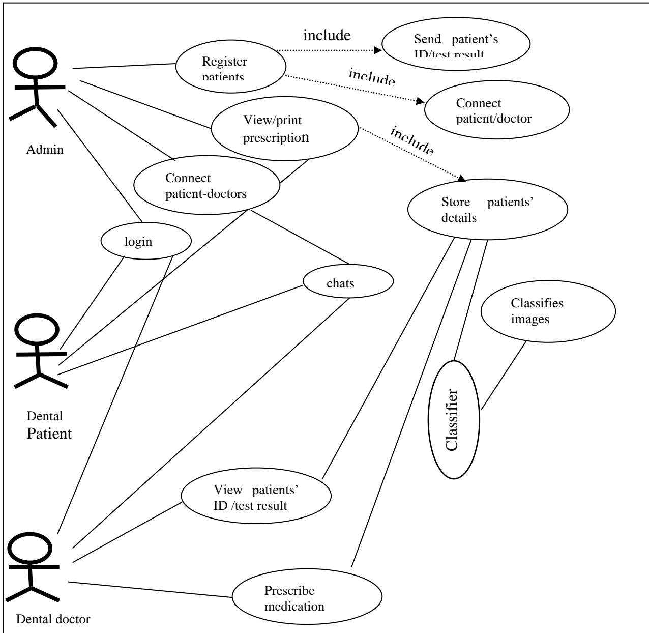
Figure 4.1 System Use-Case-Diagram
